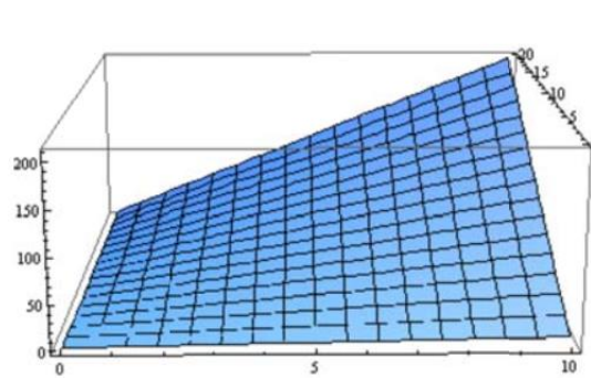
Gambar 6 Output pada interval x = \{x | 0 \leq x \leq 10\} ; t = \{t | 0 \leq t \leq 20\} .
