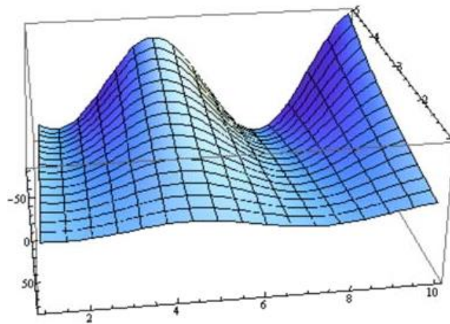
Gambar 2 Output pada interval x = \{x|1 \leq x \leq 5\}; t = \{t|1 \leq t \leq 20\} .
