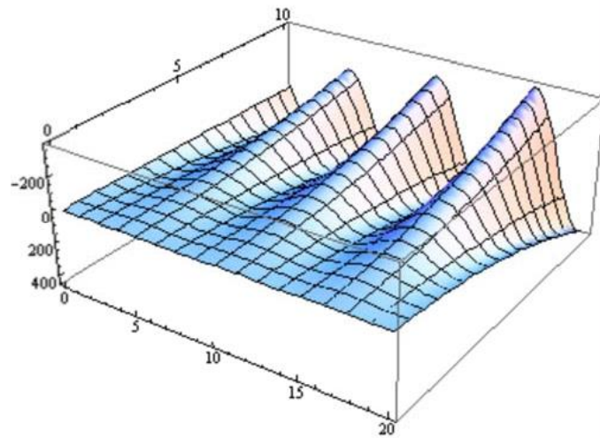
Gambar 3 Output pada interval x = \{x|0 \leq x \leq 10\}; t = \{t|0 \leq t \leq 20\} .
