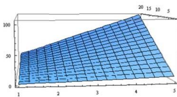
Gambar 5 Output pada interval x = \{x | 1 \leq x \leq 5\} ; t = \{t | 1 \leq t \leq 20\} .
